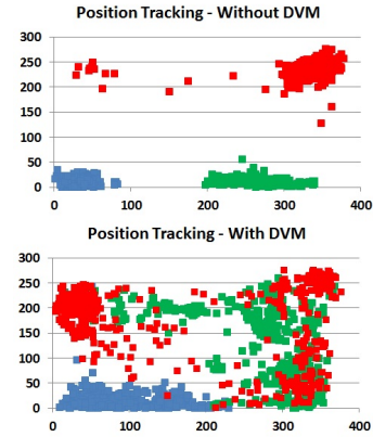
Figure 3: Overview of positions of rhythm guitarist (in red), lead guitarist (in blue) and bassist (in green) without and with DVM, sampled at 1-second intervals.
